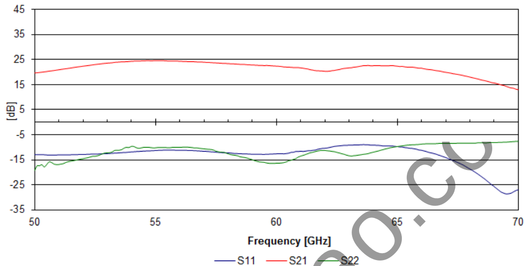
V-MPA 50-70 20 16 - Gain and Return Loss Performance
